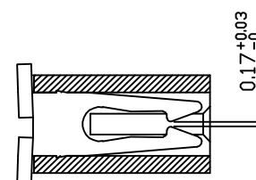
Q-Q SECTION
