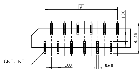
PC BOARD LAYOUT TOP VIEW PCB T=1.6mm
