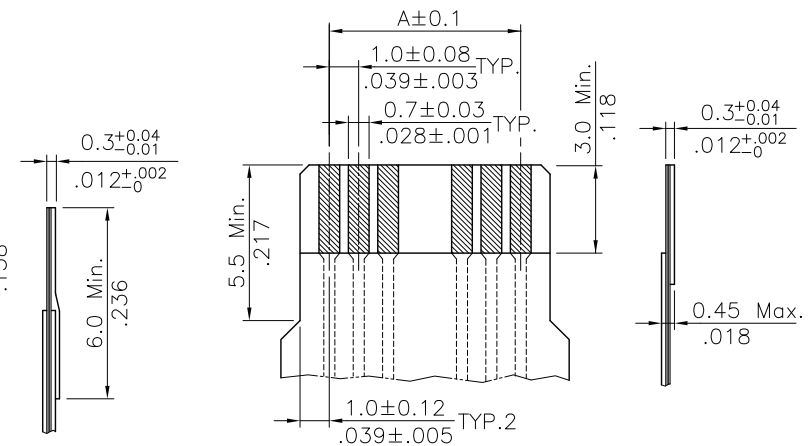
* ACCOMMODATED FPC
