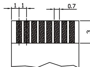
FFC/FPC DIMENSION THICKNESS 0.3mm TOLERANCE: 0.05mm
