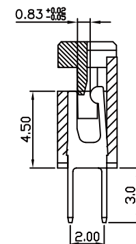
SECTION M-M
