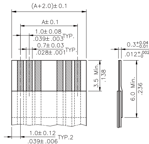
* ACCOMMODATED FFC
