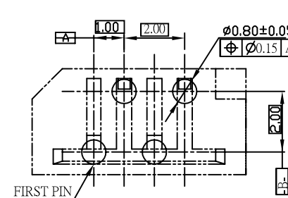
P.C.B. LAYOUT t=1.6\text{mm} COMPONENT SIDE
