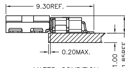
MATED CONDITION
