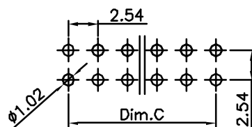
Recommended P.C.B. Layout (Tolerance:0.05mm)
