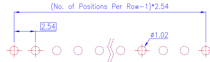
PCB Layout (Top View)
