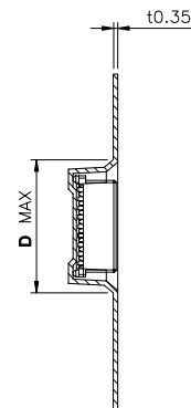
B-B SECTION
