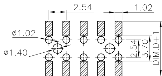
RECOMMENDED P.C.B LAYOUT FOR BOTTOM ENTRY (Tolerance:±0.05)
