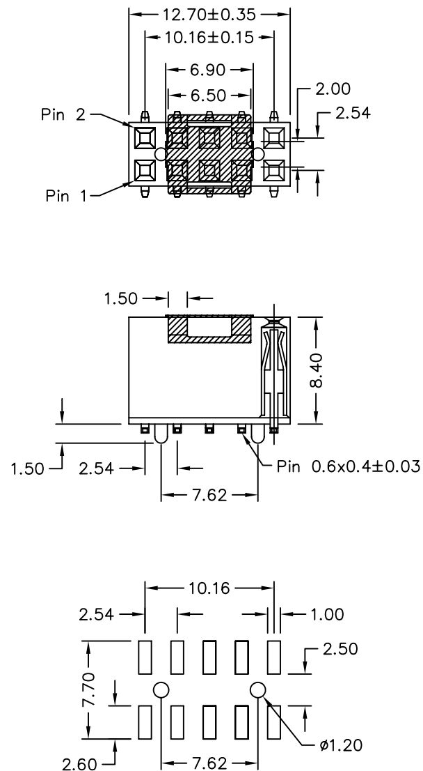
Recommended P.C.B Layout
