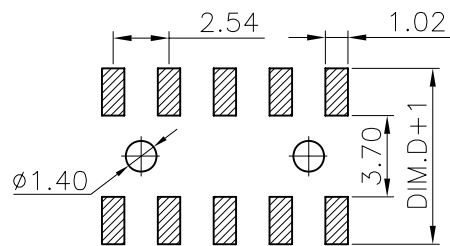
Recommended P.C. Board Layout (Tolerance: \pm 0.05 )
