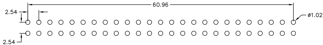
Recommended P.C.B Layout
