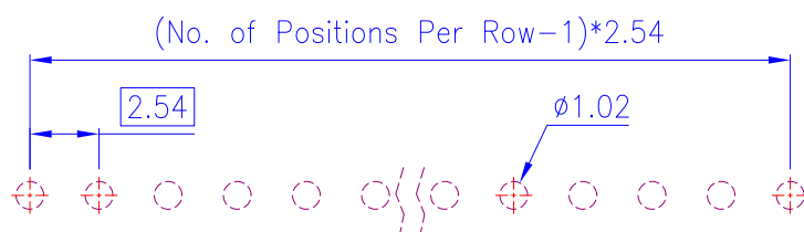
PCB Layout (Top View)
