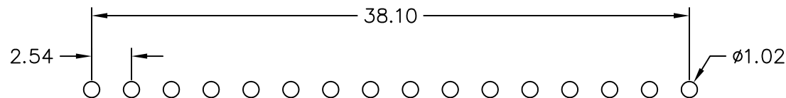
Recommended P.C.B Layout
