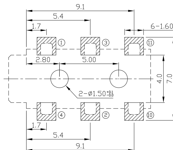
RECOMMENDED SOLDER PAD LAYOUT
