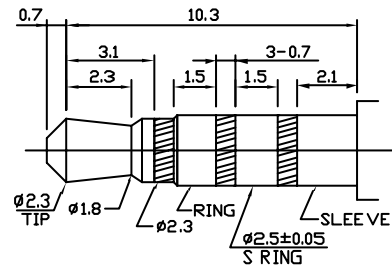
4P PLUG
