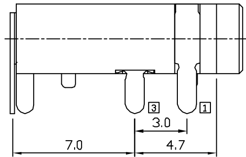
4P PLUG
