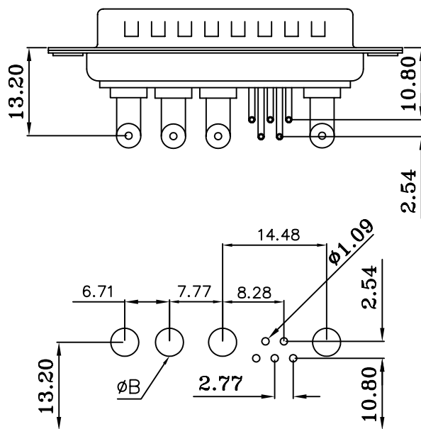
PCB LAYOUT
