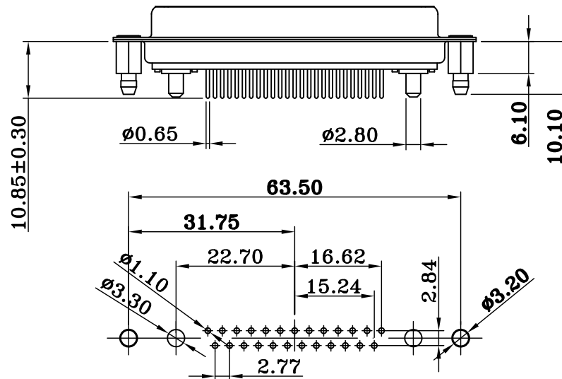
PCB LAYOUT
