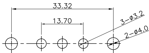
PCB LAYOUT
