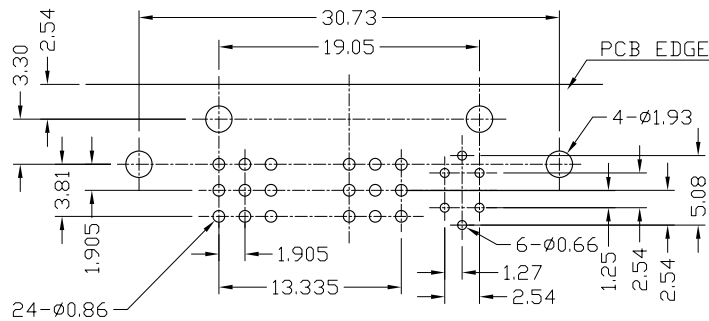
PCB LAYOUT (BOTTOM VIEW) TOLERANCE: ±0.05
