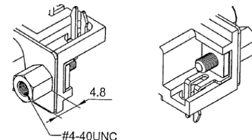
4-40 THREADED RIVETED W/BOARDLOCK AND JACK SCREWS
