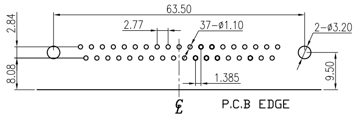
RECOMMENDED P.C.B LAYOUT INSPECTION DIMENSION:(A)~(H)
