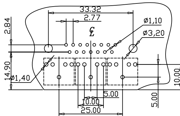
RECOMMENED P.C.B. AYDOUT
