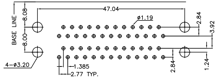
RECOMMEND P.C.B. LAYOUT BOTTOM VIEW
