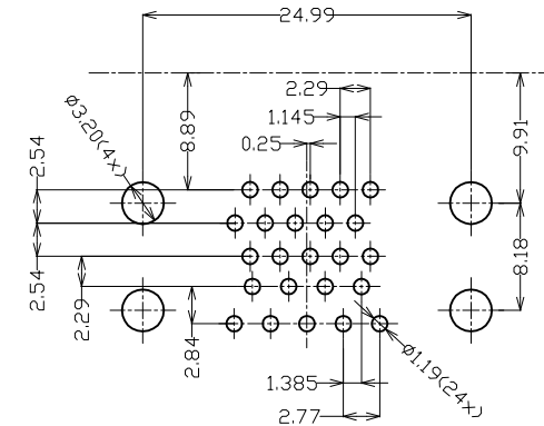
RECOMMEND P.C.B. LAYOUT BOTTOM VIEW
