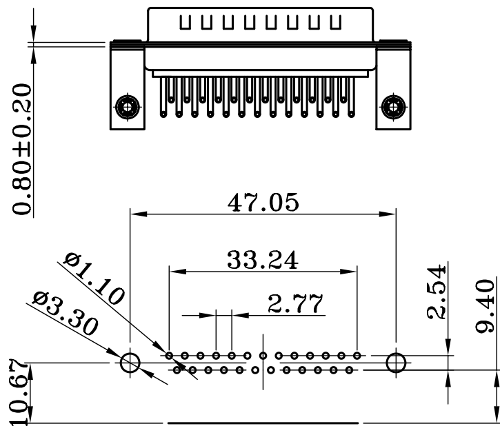
PCB LAYOUT
