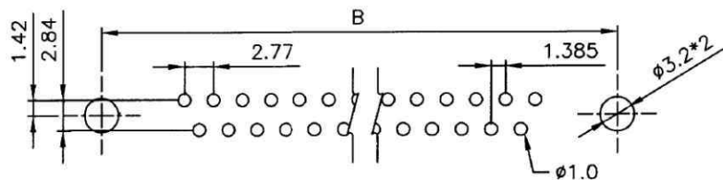
RECOMMENDED P.C.B LAYOUT (TOP VIEW) TOLERANCES: ±0.05mm
