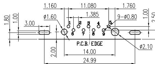
RECOMMENDED P.C.B LAYOUT INSPECTION DIMENSION:(A)~(I)
