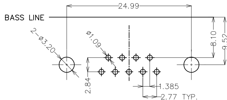
P.C.B. LAYOUT(TOLERANCE±0.05) TOP VIEW
