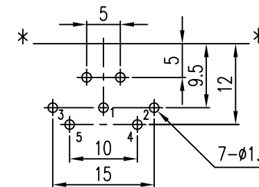
RECOMMEND PCB HOLES LAYOUT
