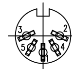
PIN LAYOUT ( TO INSERT PIUG )
