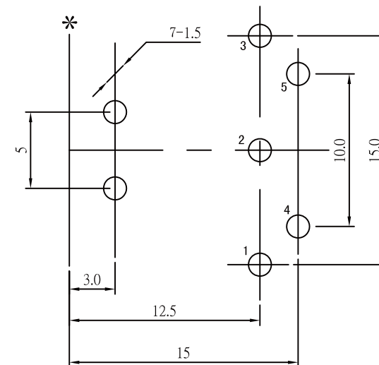
T:1.6 Dimensions of PC board holes Tolerance : \pm 0.1 (Printed-top view)
