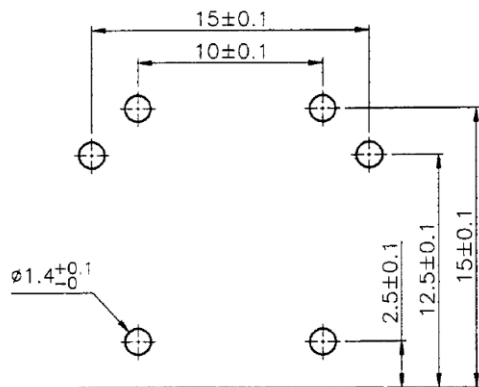
PCB HOLE PATTERN (TOP VIEW)
