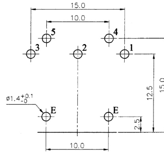
PCB LAYOYT (TOP VIEW)
