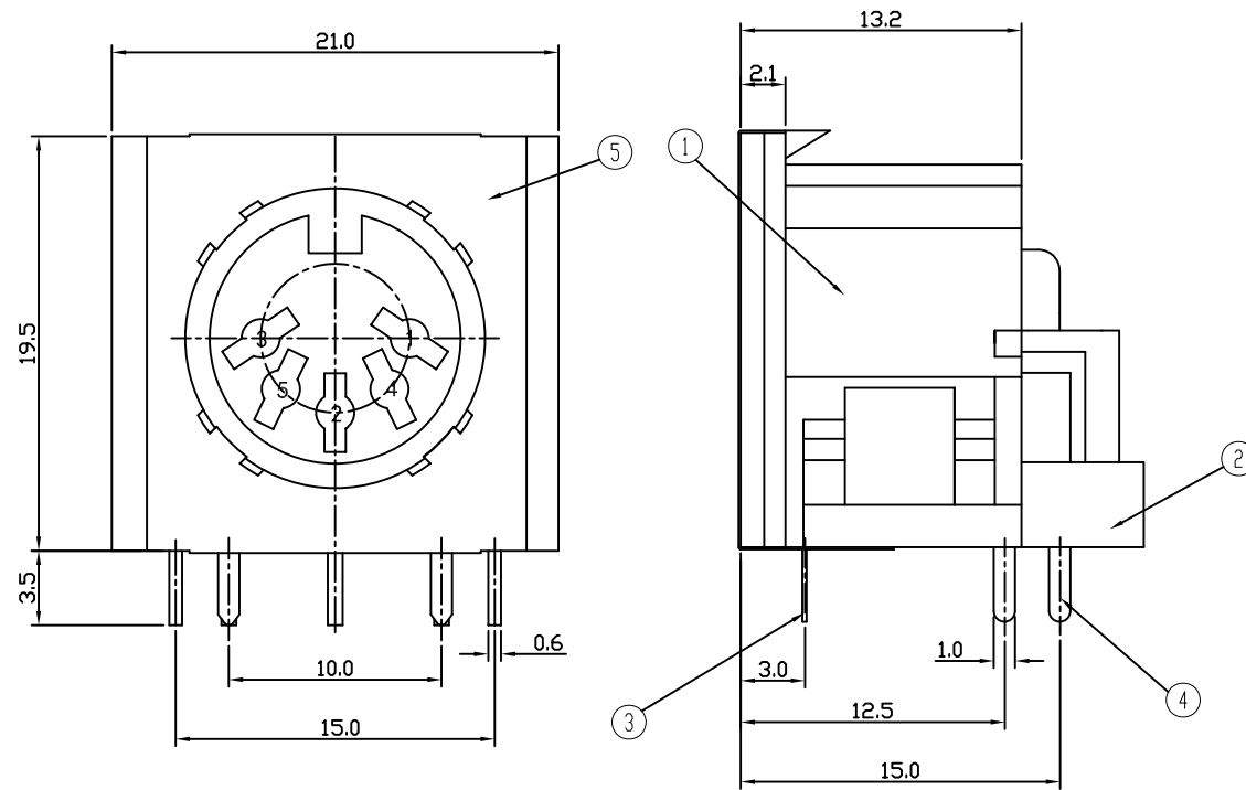
T:1.6 Dimensions of PC board holes
