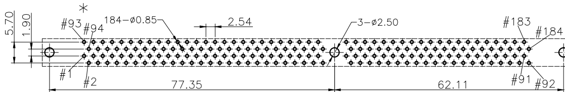
TOP VIEW PCB LAYOUT RECOMMENDED
