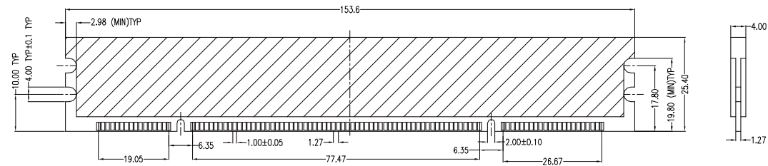
Recommended Daughter Card
