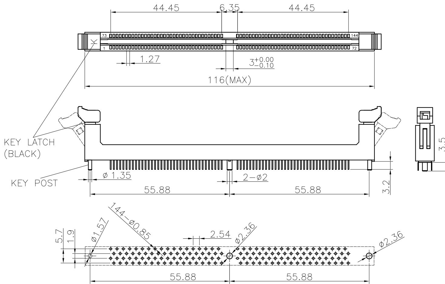
TOP VIEW PCB LAYOUT RECOMMENDED
