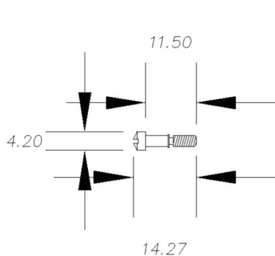
screw #4-11.5-0.5 UNC 4-40
