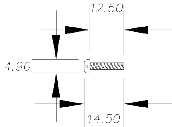
screw #4-12.5 UNC 4-40
