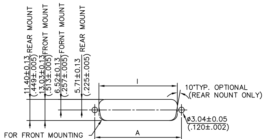
RECOMMENDED PANEL CUTOUT DIMENSIONS
