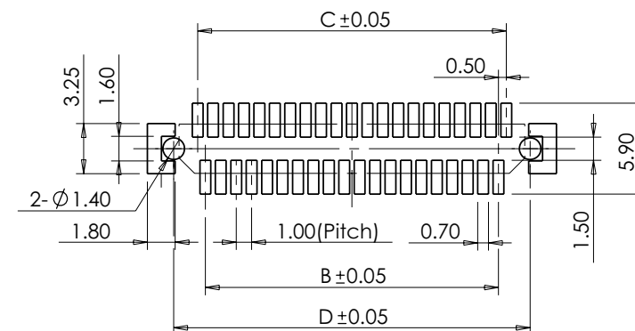
PCB Layout(REF.) Component Top View
