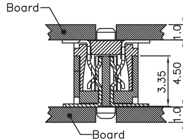
Mating Drawing (Ref.)
