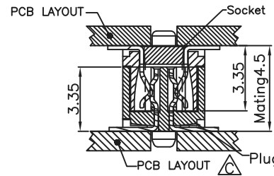
Mating Drawing (Ref.)
