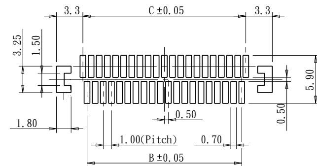
PCB Layout(REF.) Component Top View
