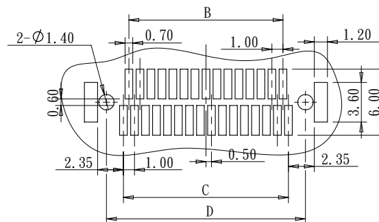
PCB Layout(REF.) Component Top View
