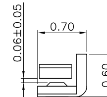
Section C-C(SCALE 2:1)
