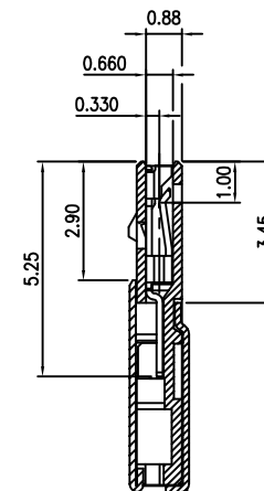
SEC.A-A SCALE 8:1
