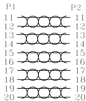
WIRING DIAGRAM
