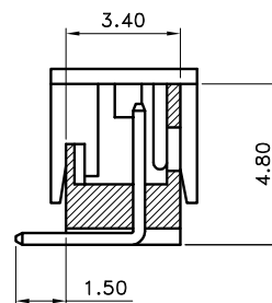
A-A Section plane
